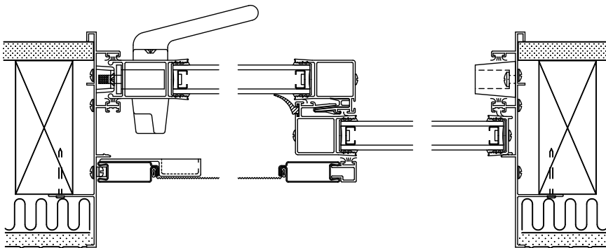
SHOWING 5 1/4" FRAME DUAL GLAZED
