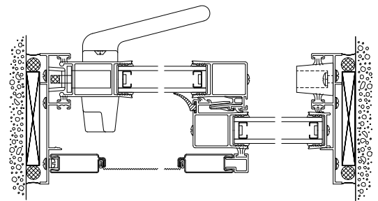
HORIZONTAL SECTION - 6980 SERIES
